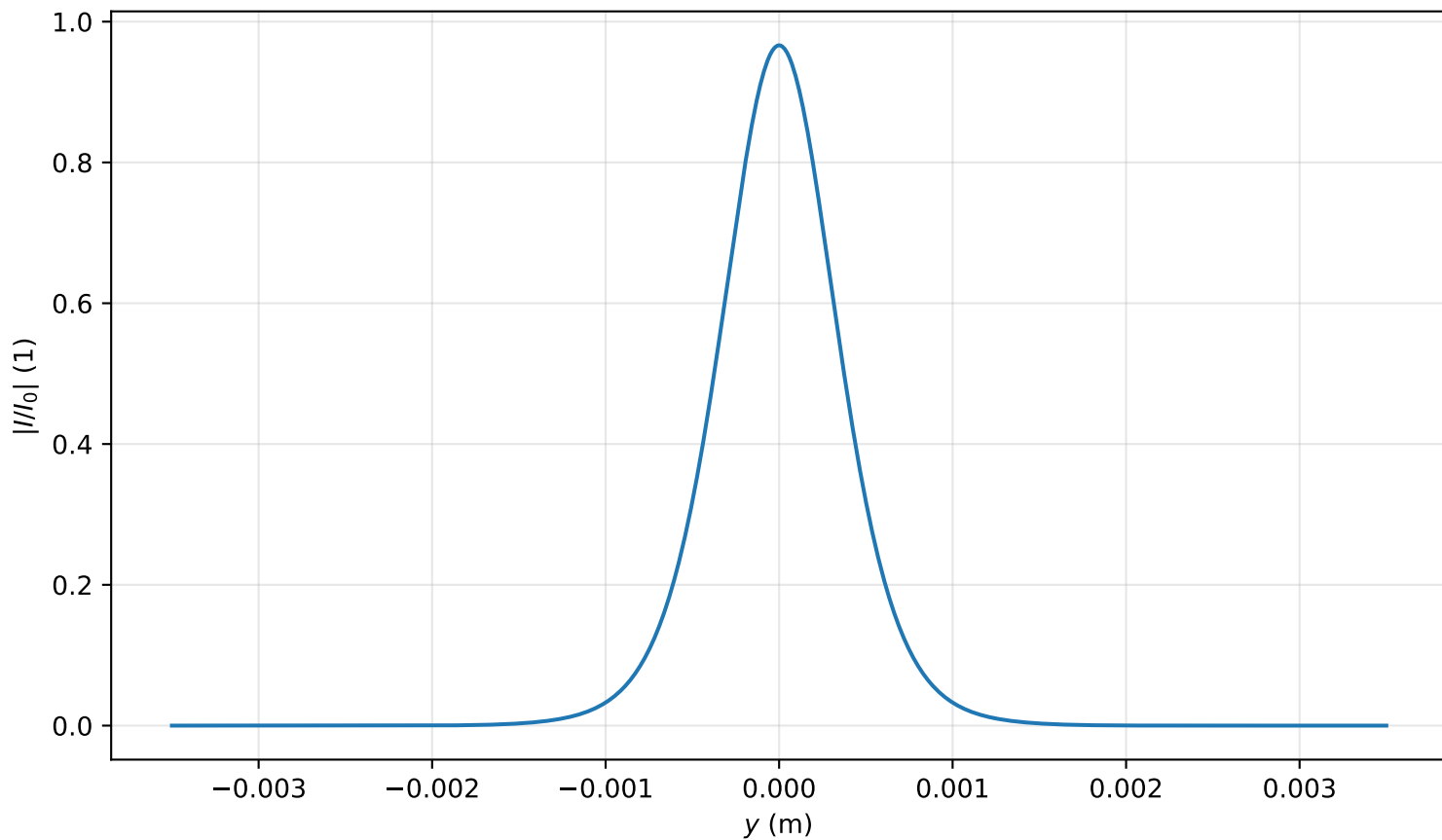
Intensity profile I(x=0, y, z=1.911)/I_0 , P_{in}=0.6P_{cr} , artificial time
